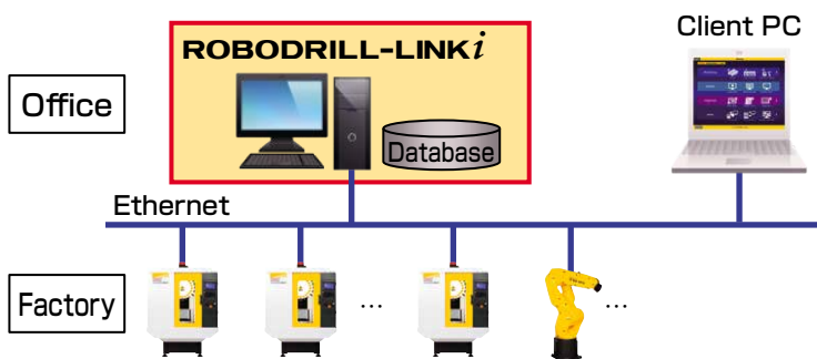
Connection example
